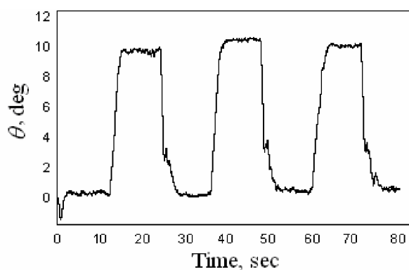
Fig. 6. Flight trajectory angle variations (0,9m)
