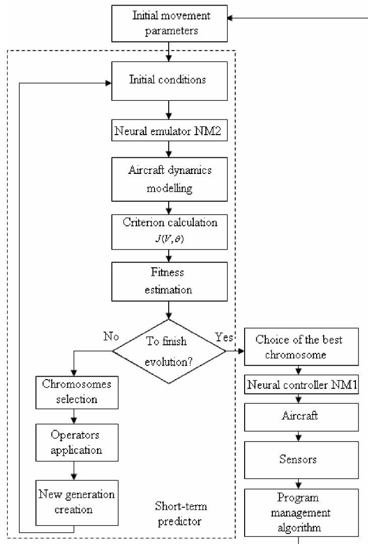
Fig. 2. Algorithm operation flow-chart
