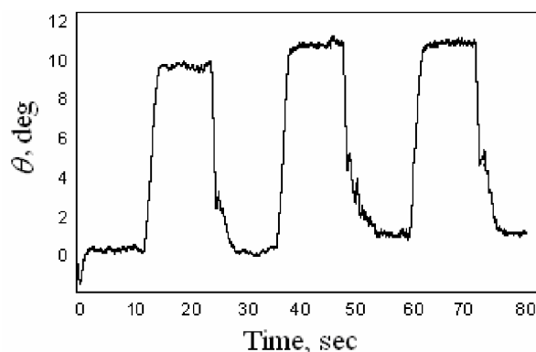
Fig.7. Flight trajectory angle variations (0,75m)
