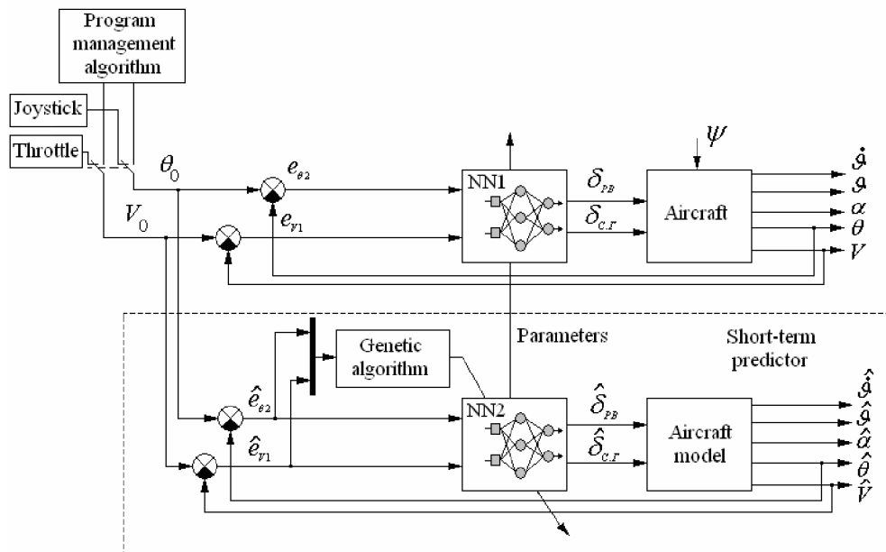
Fig. 1. General structure of the control system
