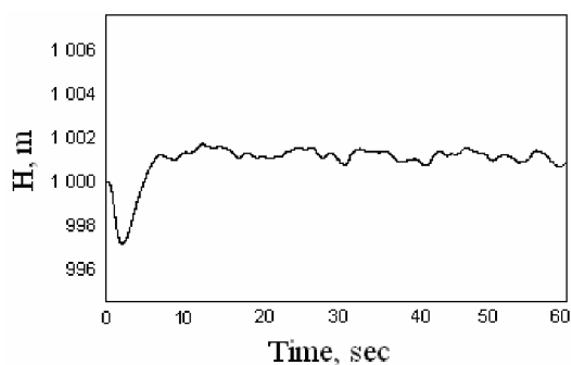
Fig. 4. Maintaining constant altitude
